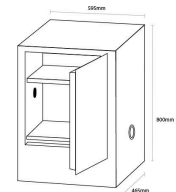
External Size: 800(H) x 550(W) x 400(D)mm Internal Size: 600(H) x 350(W) x 370(D)mm
